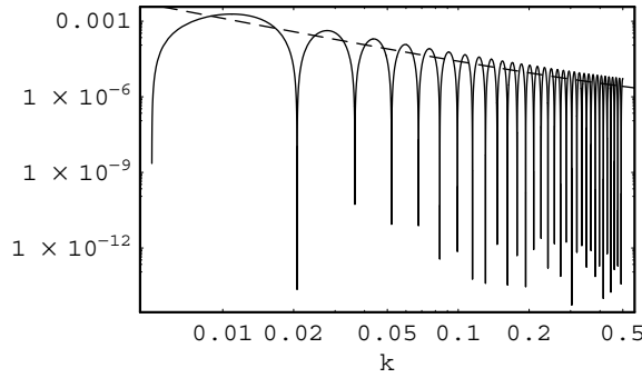
Figure 1. n(k) - 1 as function of k (solid curve), with \eta^* = -200 , and \lambda = 10^{-3} . The dashed curve shows n(k) - 1 once the rapidly oscillatory terms have been removed. The main departures from zero come from the mass term induced by the coarse graining.
